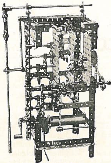
Clock Mechanism
