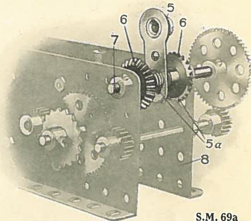
S.M. 69a Detail of Drive-Changing Gear (S.M. 69)
